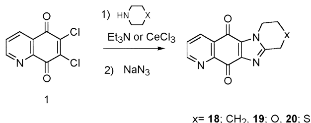
Figure 3. Scheme of the synthetic method of the tetracyclic imidazoquinolinedione derivatives, 18 , 19 and 20 .
