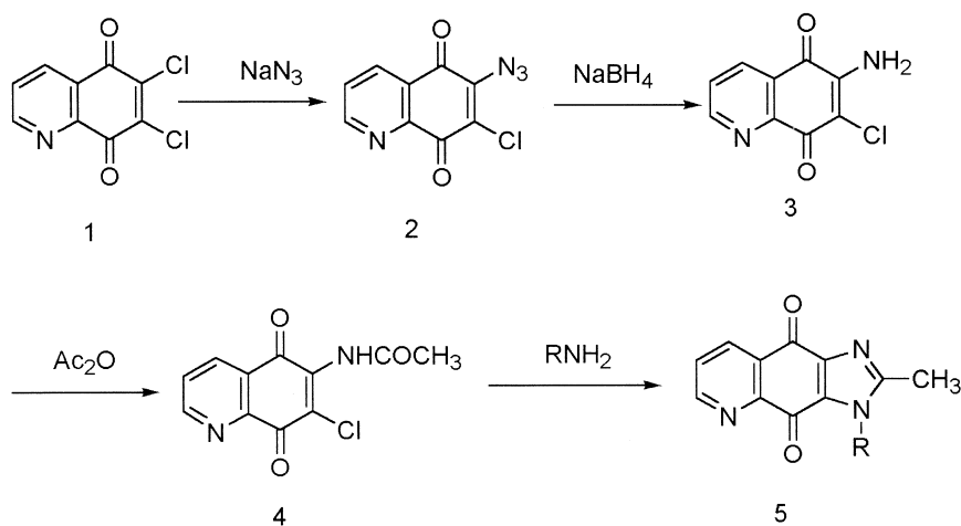
Figure 2. Scheme of the synthetic method of 1-alkyl-imidazoquinoline-4,9-diones ( 5–12 ) and 1-aryl-imidazoquinoline-4,9-dione ( 13–17 ). R = 5 : methyl, 6 : ethyl, 7 : propyl, 8 : butyl, 9 : chloroethyl, 10 : \beta -hydroxyethyl, 11 : isopropyl, 12 : benzyl, 13 : phenyl, 14 : 4-bromophenyl, 15 : 4-ethoxyphenyl, 16 : 4-chlorophenyl, 17 : 4-methylphenyl.
