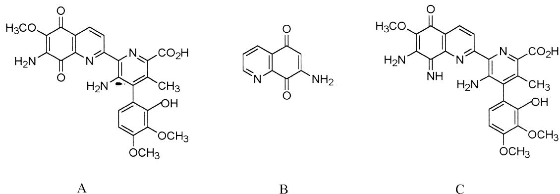
Figure 1. Streptonigrin structure (A), 7-aminoquinolinequinone moiety (B) that is responsible for the antitumor activity of streptonigrin and azastreptonigrin (C).
